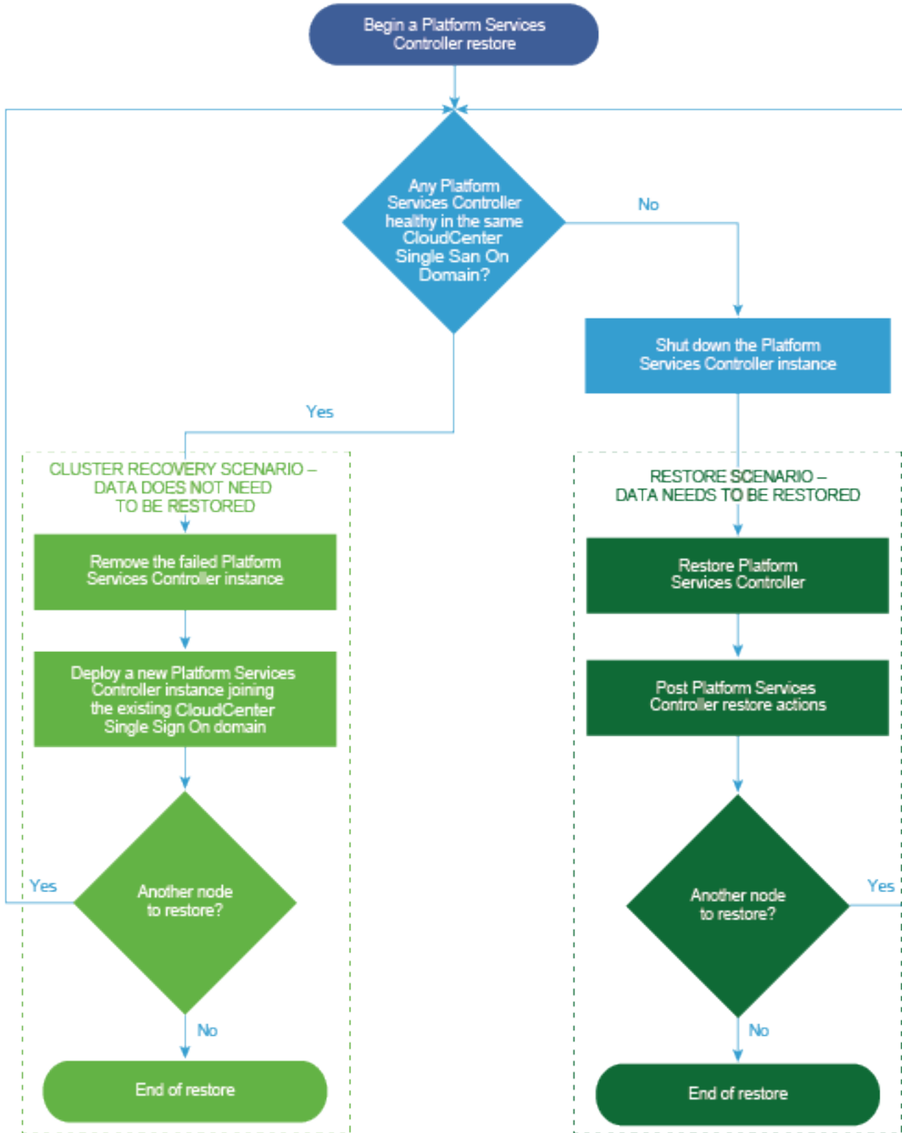
图 7-2 Platform Services Controller 还原 workflow
