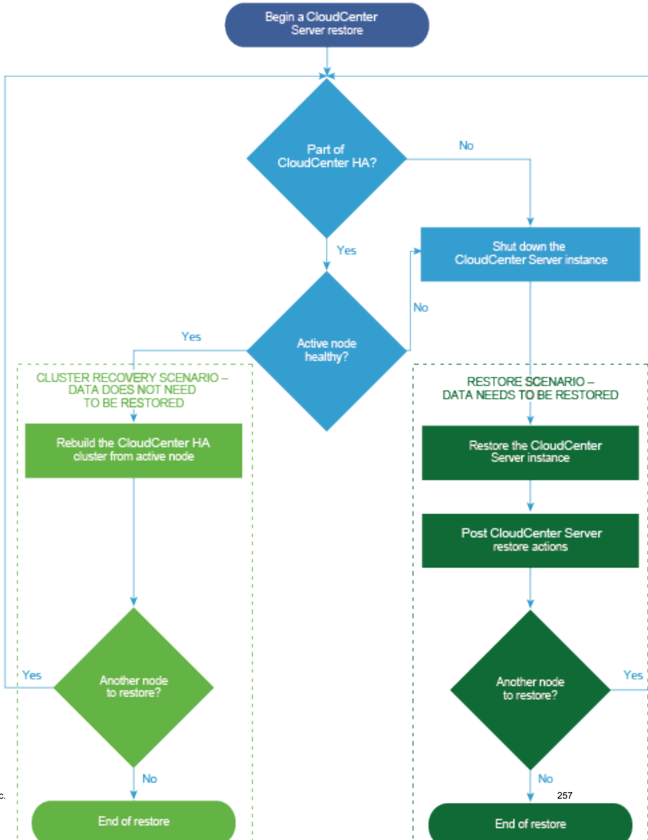
图 6-1 vCenter Server Appliance 还原 workflow
