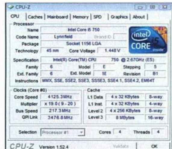
酷睿i5 750处理器配合SABERTOOTH 55i轻松超频到4.1GHz
