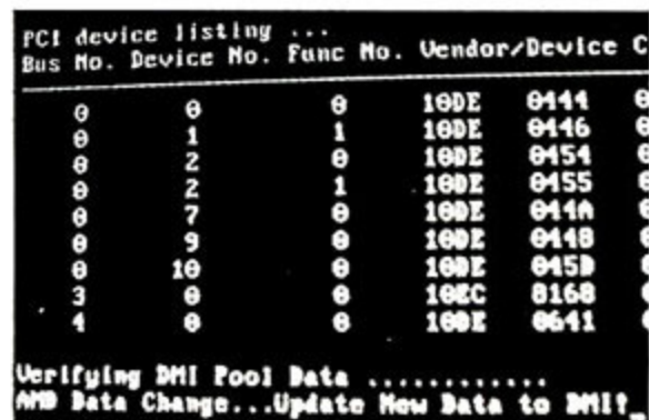
启动时提示AMD data changed
