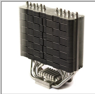
● 拆掉风扇后,散热片看上去很单薄
